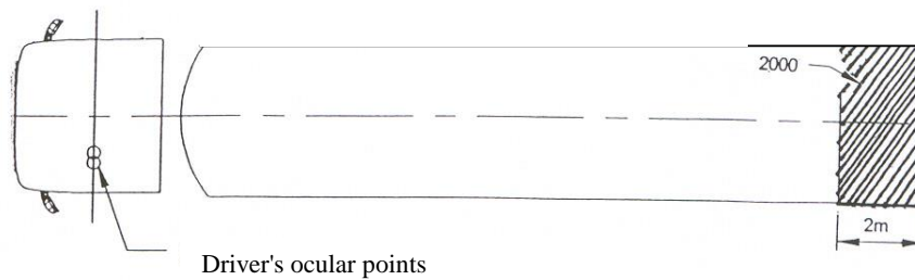
Figure 12 : Field of vision of rear devices for indirect vision
