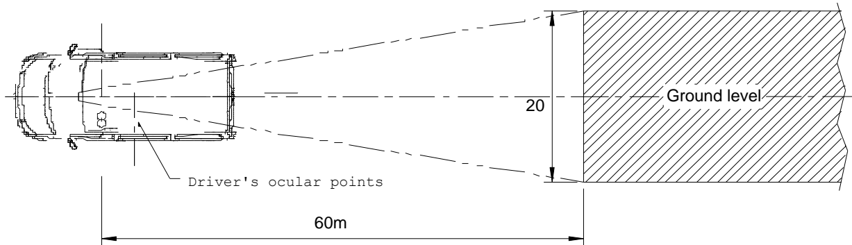
Figure 6: Field of vision of Class I mirror
