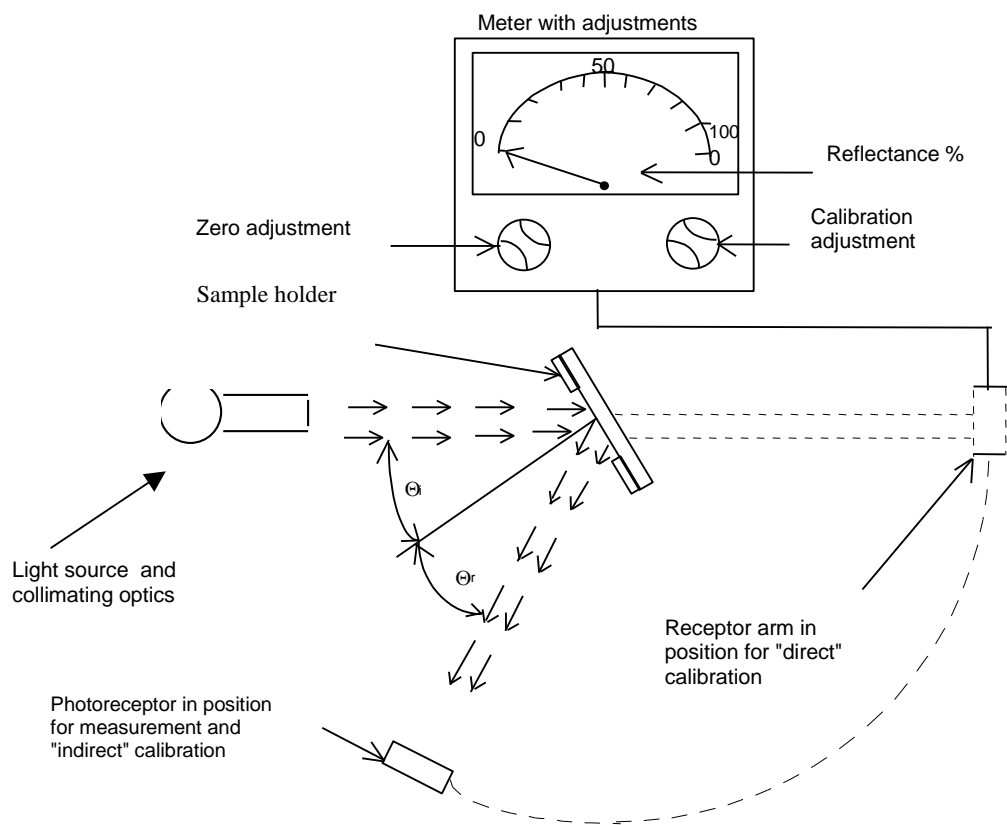
Figure 4 Generalised reflectometer showing experimental set-ups for the two calibration methods
