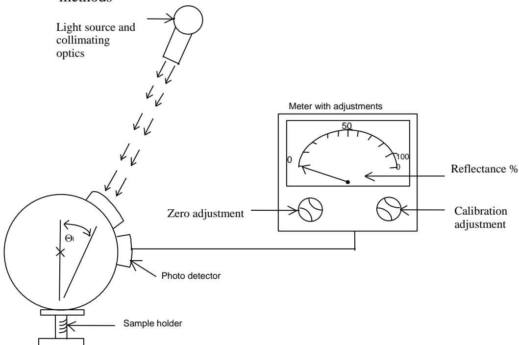
Figure 4 Generalised reflectometer showing experimental set-ups for the two calibration methods
