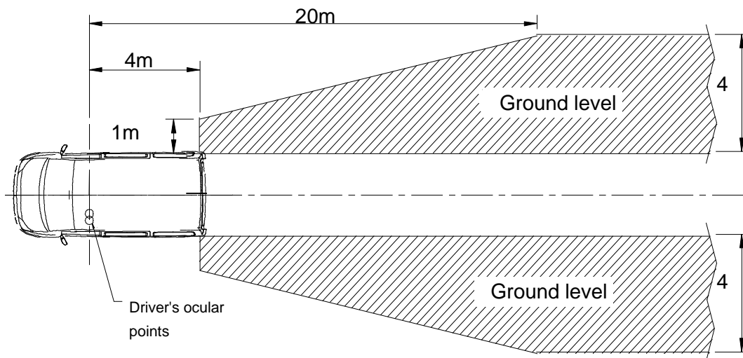
Figure 8: Field of vision of Class III mirrors
