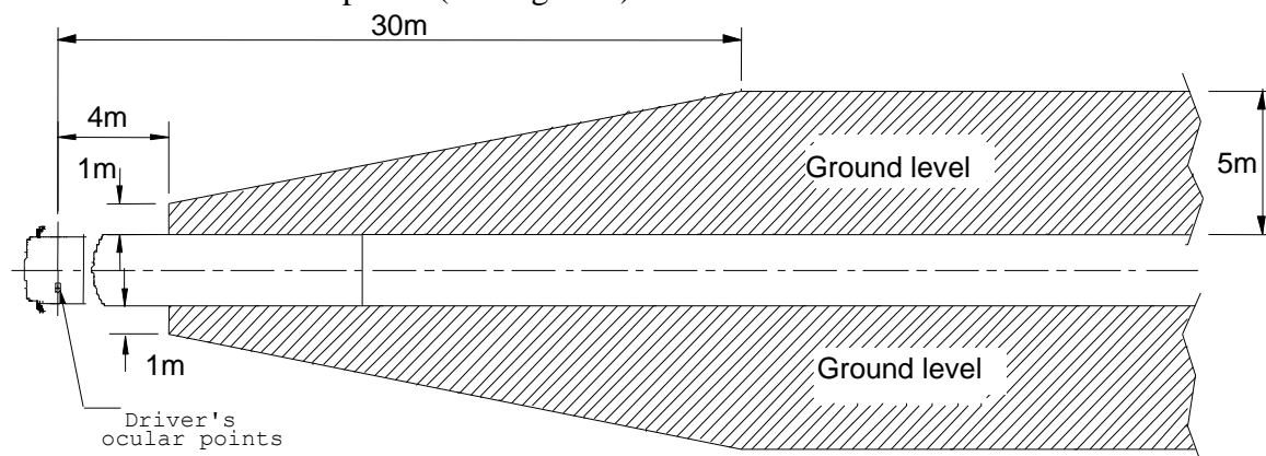
Figure 7: Field of vision of Class II mirrors
