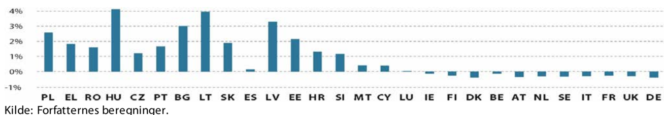
Figur 2. Driftsbudgetsaldoer (%BNI, 2018)
